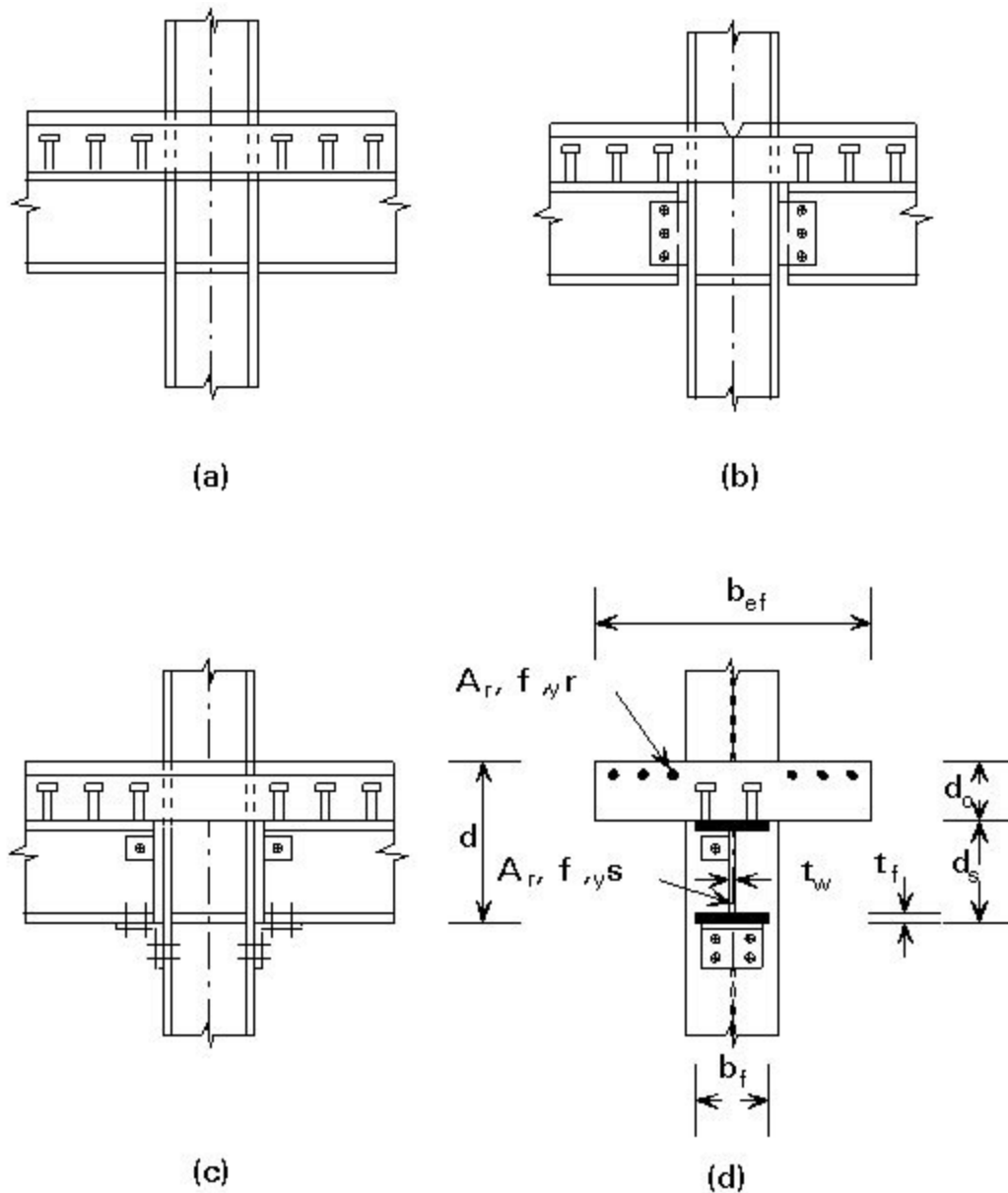
Figure 11 – Composite Joints
