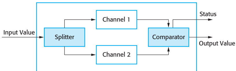
Figure 13.4 Self-monitoring architecture
