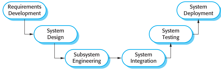
Figure 10.7 Systems development
