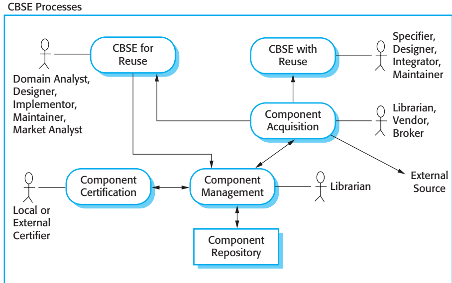
Figure 17.6 CBSE processes
