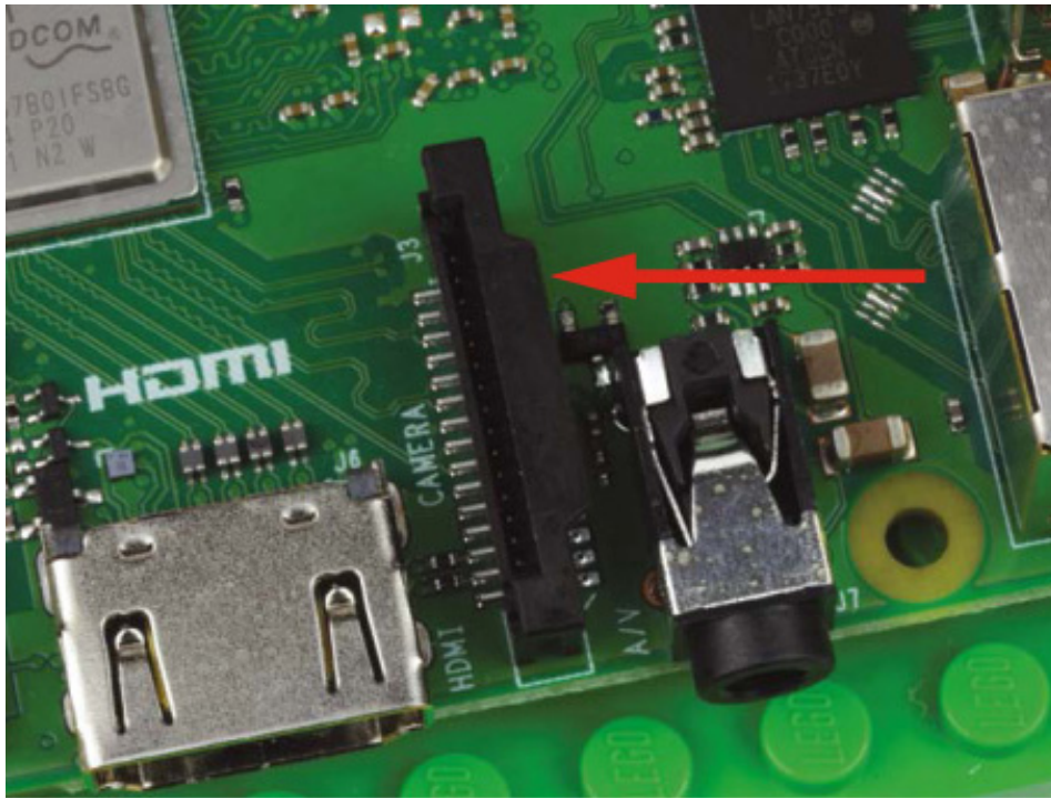
FIGURE 8-3 The CSI interface port on the Raspberry Pi
