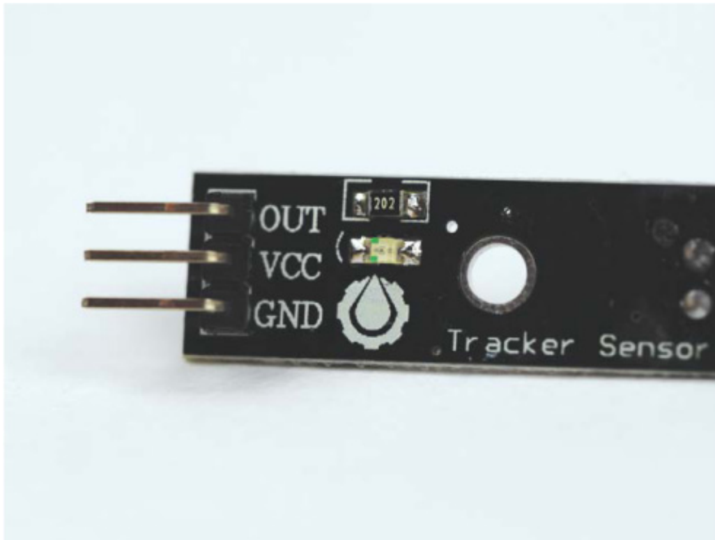
FIGURE 7-10 Pinout of a TCRT5000 IR sensor module
