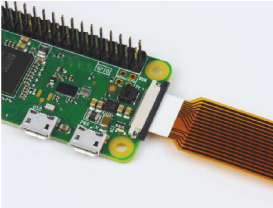
FIGURE 8-7 The correct orientation of the camera cable for the mini-CSI port on Pi Zero models
