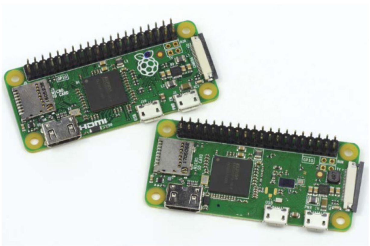
FIGURE 1-2 The Raspberry Pi Zero (left) and Raspberry Pi Zero W (right)
