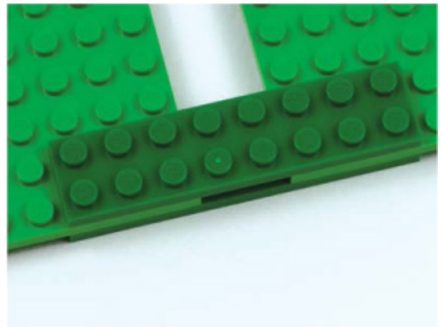
FIGURE 3-11 The completed LEGO chassis: on the right is a close-up of the joints made with the 2×8 plates
