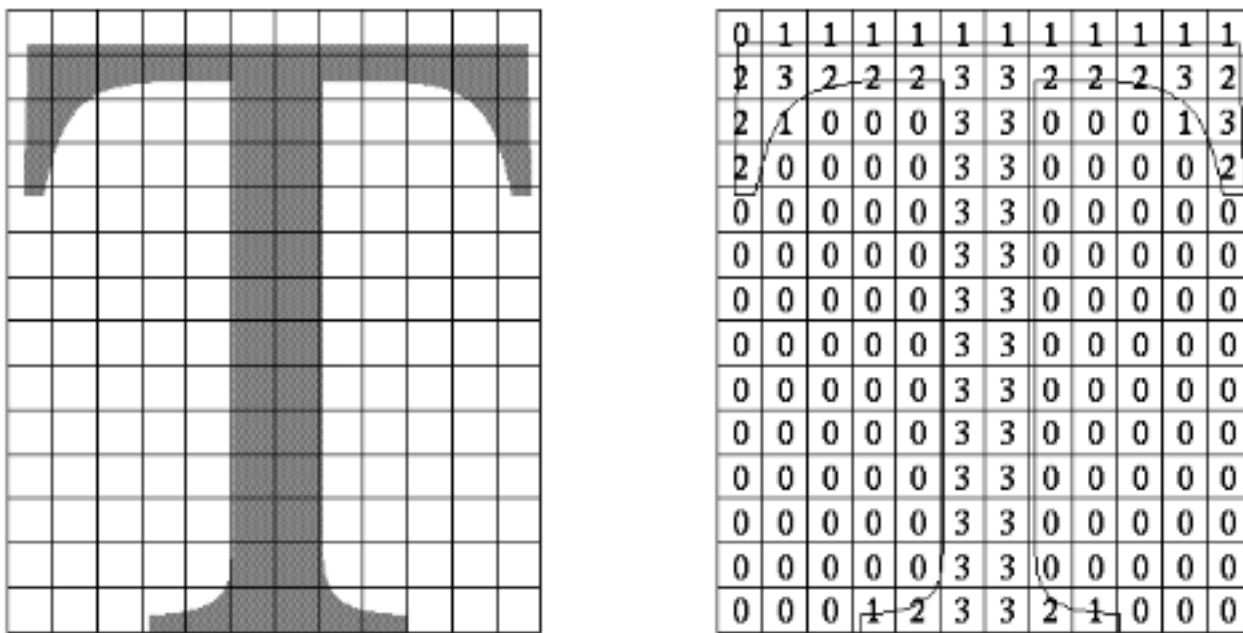
Figure 14-1 : Antialiased Characters
