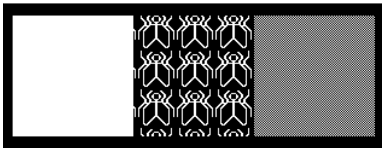
Figure 2-11 : Stippled Polygons
