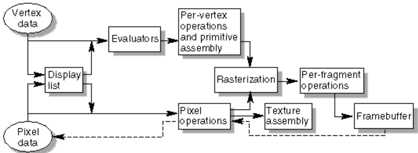
Figure 1-2 : Order of Operations
