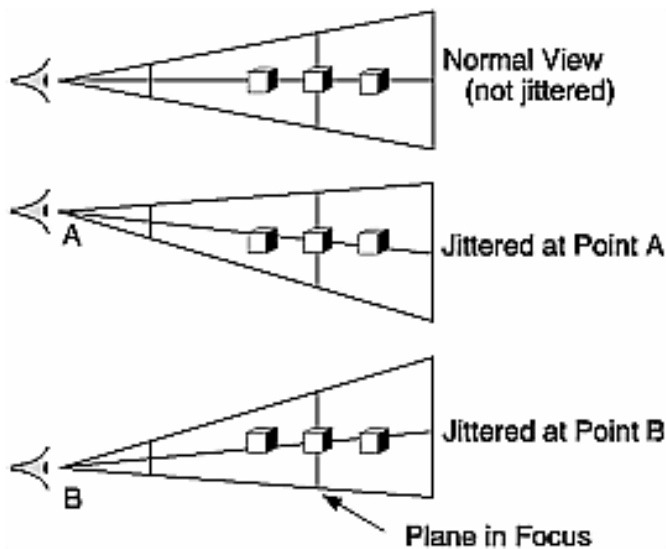
Figure 10-3 : Jittered Viewing Volume for Depth-of-Field Effects
