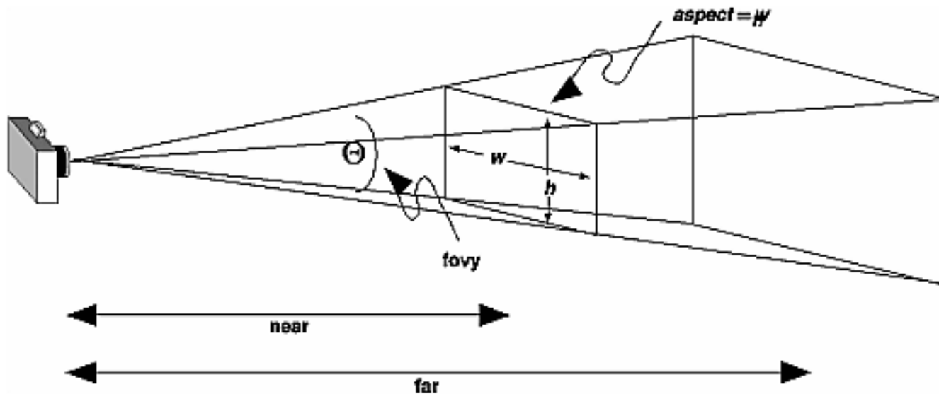
Figure 3-14 : Perspective Viewing Volume Specified by gluPerspective()
