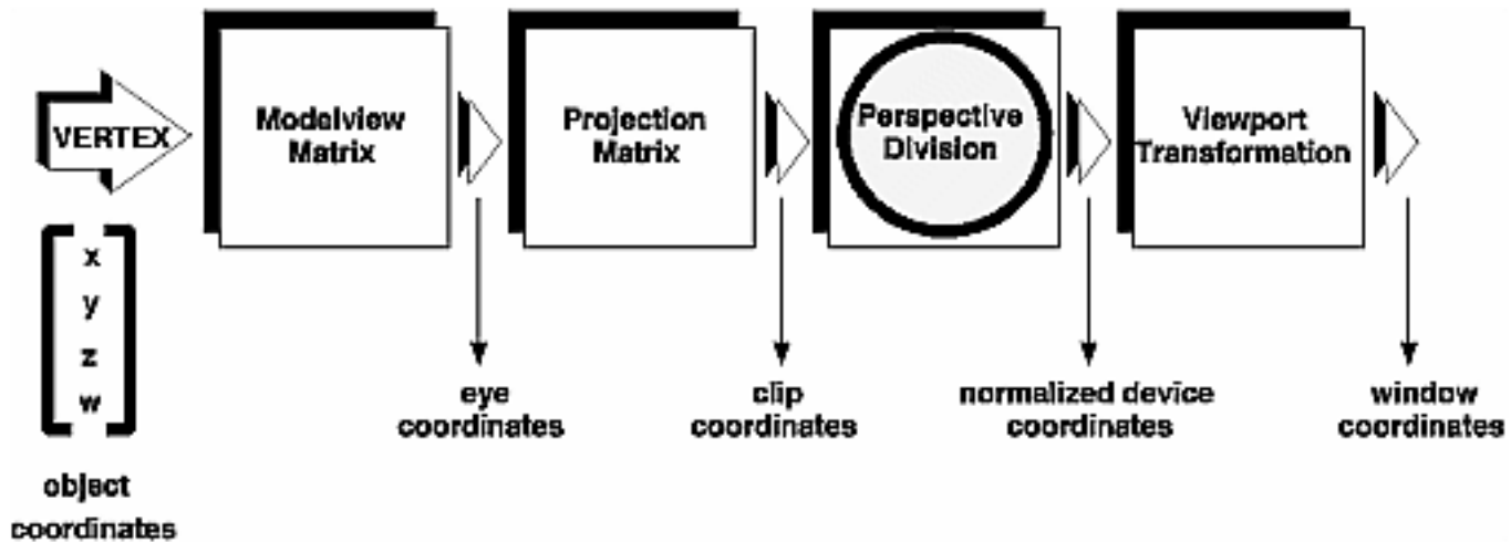
Figure 3-2 : Stages of Vertex Transformation
