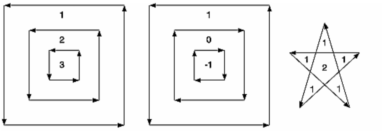
Figure 11-2 : Winding Numbers for Sample Contours
