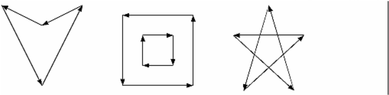
Figure 11-1 : Contours That Require Tessellation
