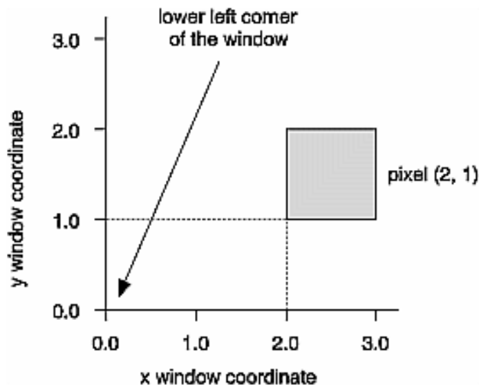
Figure 10-1 : Region Occupied by a Pixel
