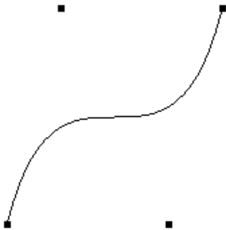
Figure 12-1 : Bezier Curve
