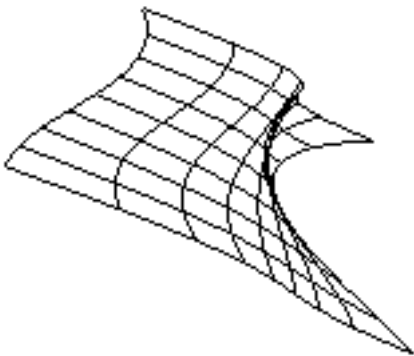
Figure 12-2 : Bezier Surface
