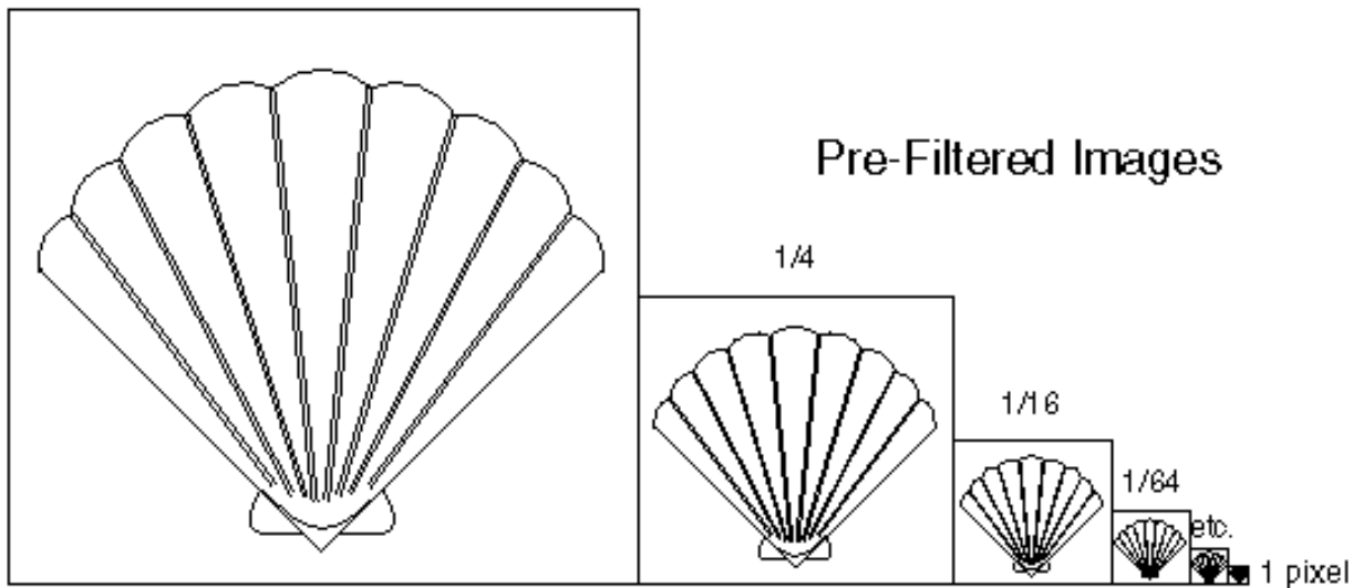
Figure 9-4 : Mipmaps
