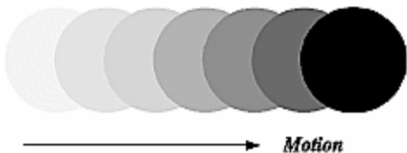
Figure 10-2 : Motion-Blurred Object
