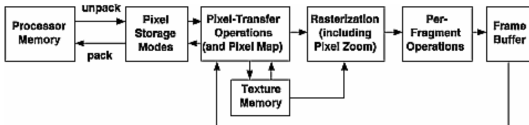
Figure 8-4 : Imaging Pipeline
