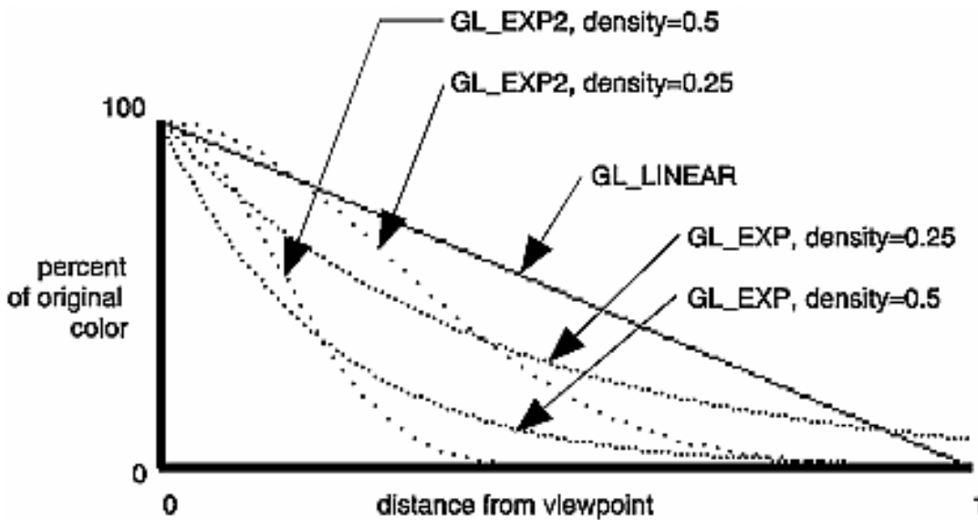
Figure 6-4 : Fog-Density Equations
