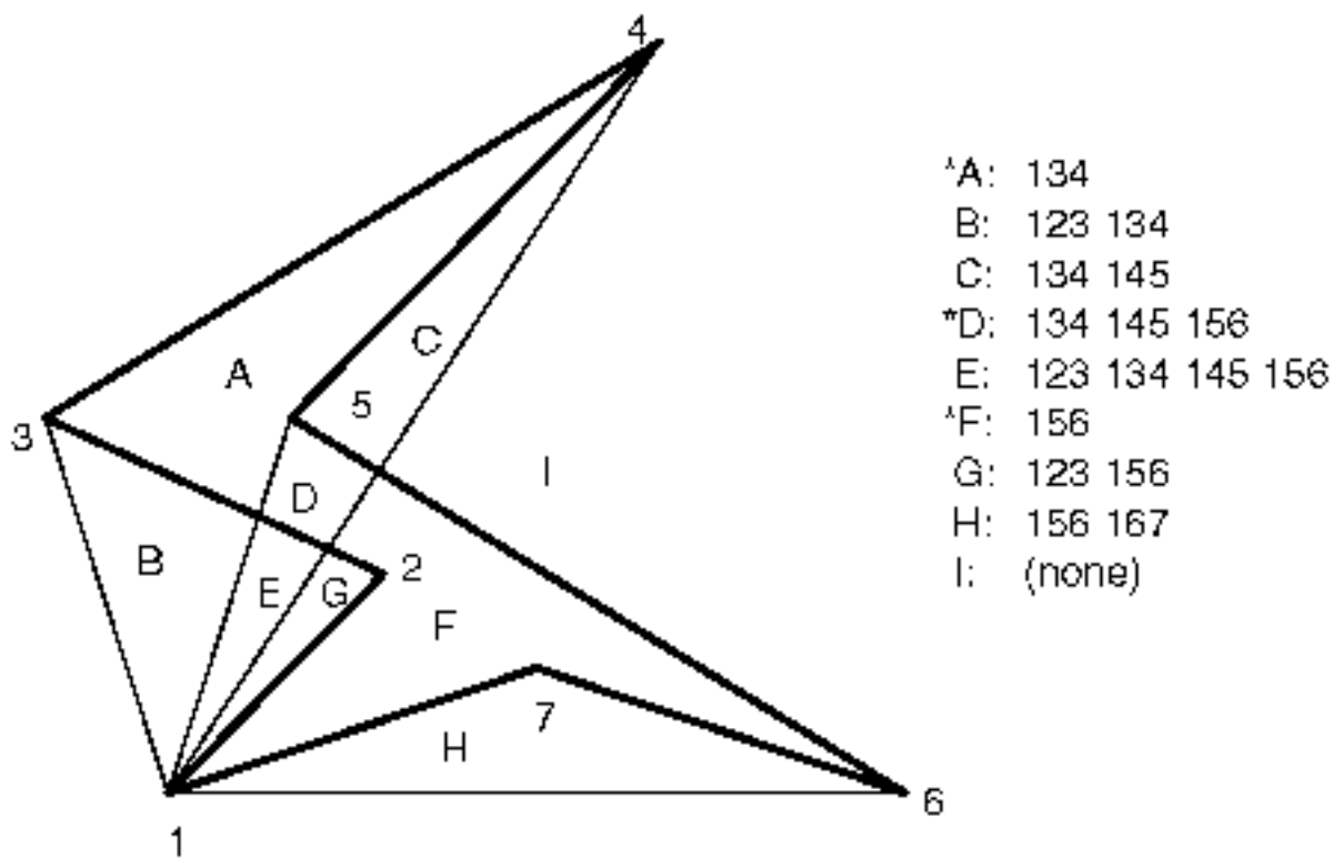
Figure 14-2 : Concave Polygon
