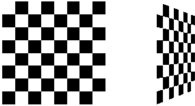
Figure 9-2 : Texture-Mapped Squares
