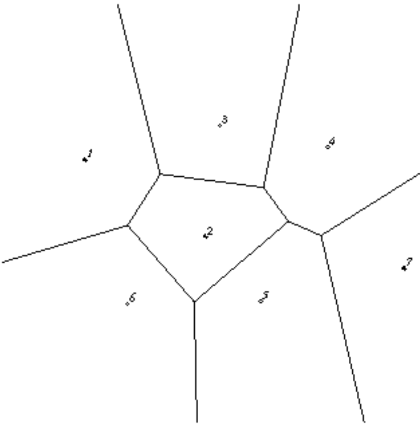
Figure 14-3 : Dirichlet Domains
