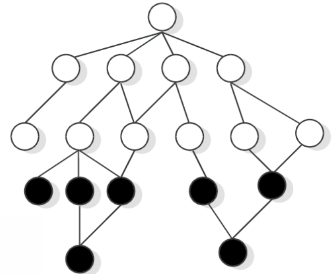
Bottom-up integration
