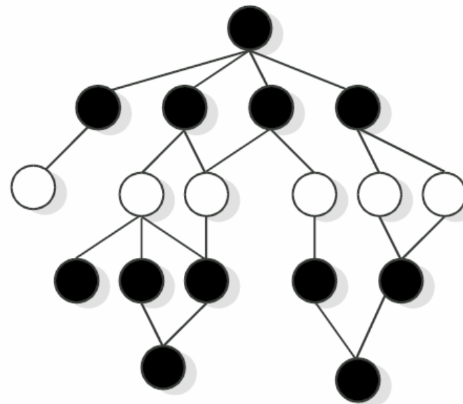
Sandwich integration
