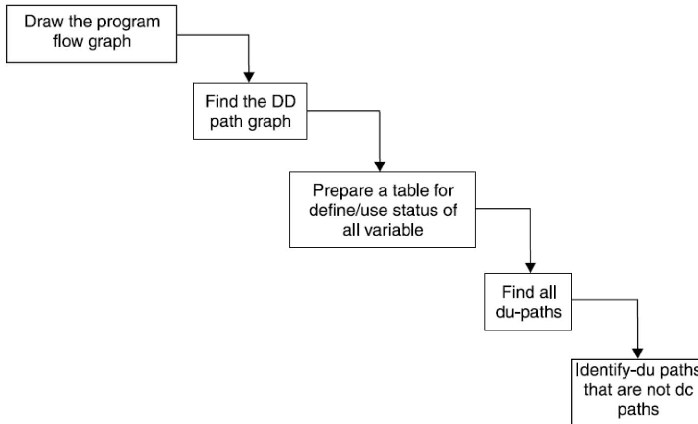
Fig. 27 : Steps for data flow testing
