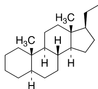
5 \alpha -Pregnane
