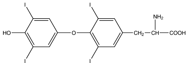
Dextrothyroxine (Choloxin)
