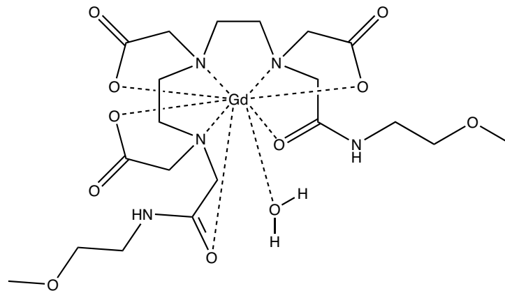
Gadoversetamide
