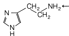
Histamine
