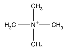
Tetramethylammonium
