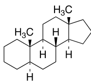
5 \alpha -Androstane
