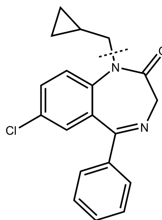
Prazepam
