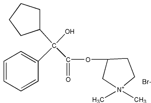
Glycopyrrolate
