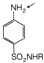
Sulfanilamide
