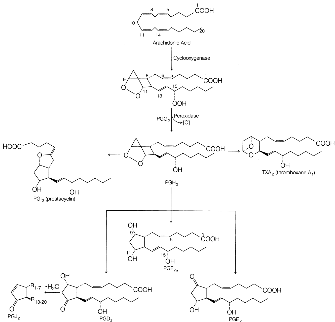
Figure 26.1 • Cyclooxygenase pathway.
