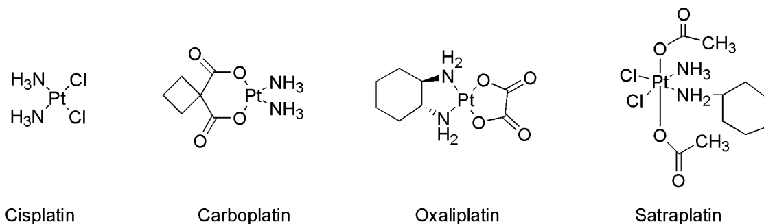
Figure 10.5 • Platinum-containing antineoplastics.
