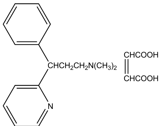
Pheniramine Maleate
