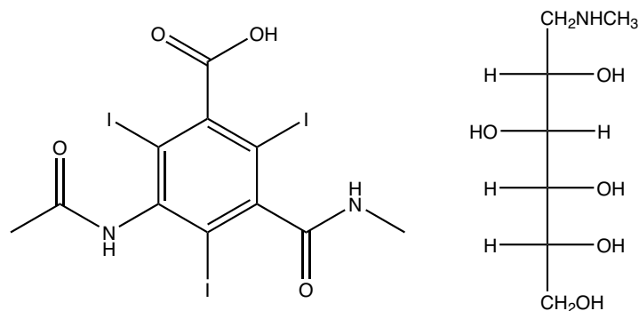
Iothalamate Meglumine
