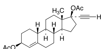
Ethynodiol diacetate
