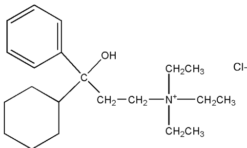
Tridihexethyl Chloride
