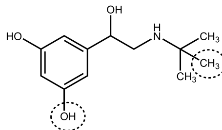
Terbutaline
