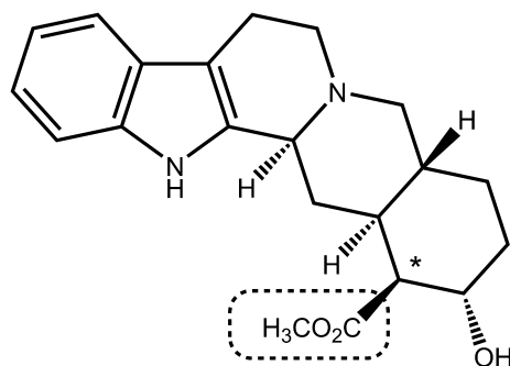
Corynanthine
