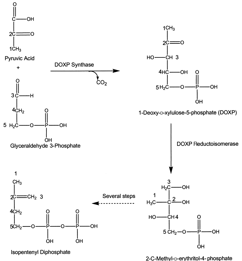
Figure 7.11 • Nonmevalonate pathway.
