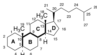
5 \alpha -Cholestane
