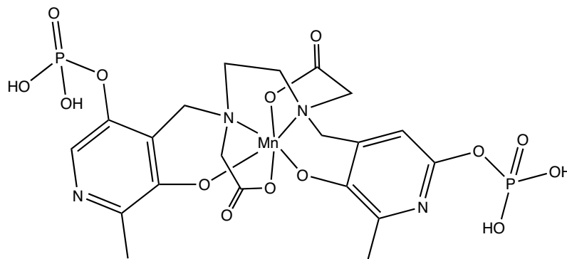
Mangafodipir
