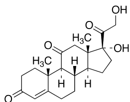
Cortisone (17,21-Dihydroxypregn-4-ene-3,11,20-trione)
