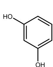
Resorcinol
