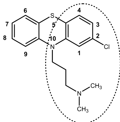
Phenthiazine
