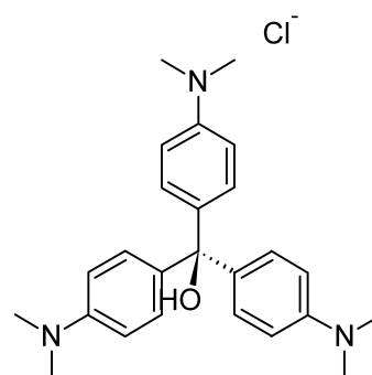
Leucobase
