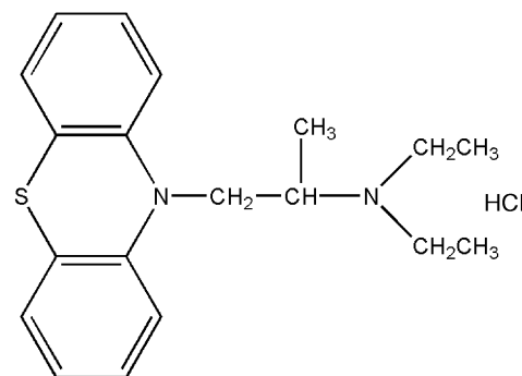
Ethopropazine Hydrochloride
