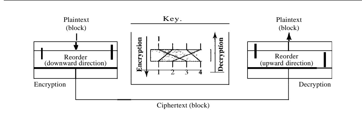
Figure 30.8 Transposition cipher
