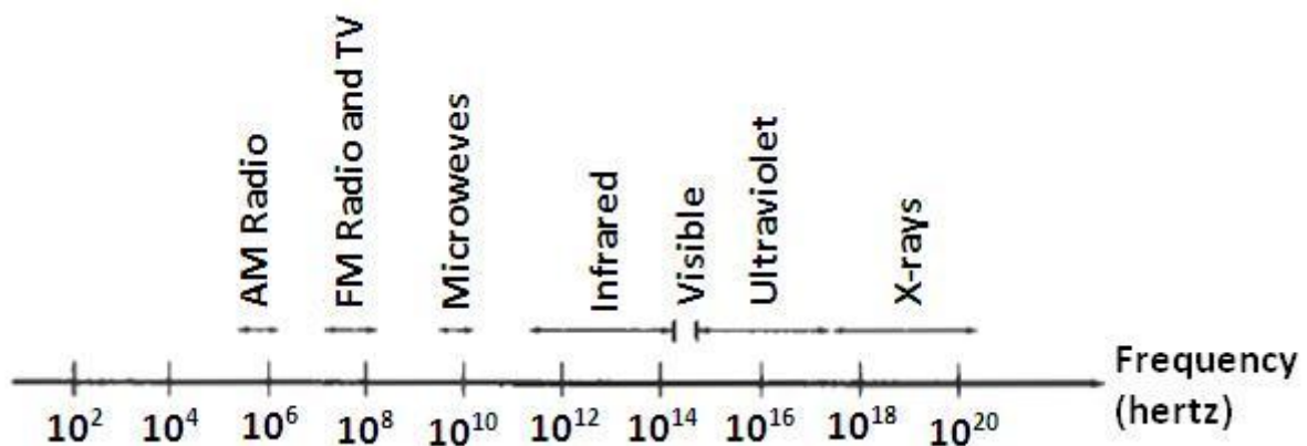
Fig. 6.11:- Electromagnetic spectrum.
